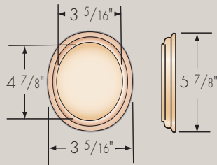
F7037 Step Detail
