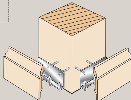
L-Anchor Newel Fastener
