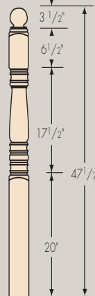
FH4500 3-1/4"
