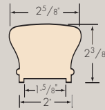
FH6210-Plow 1-5/8" Plow FH6007 Fillet
